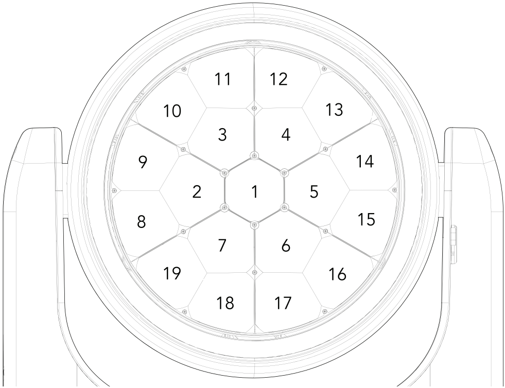
PIXEL LAYOUT
